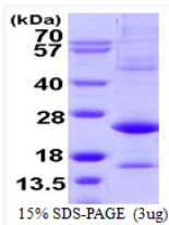
SDS-PAGE gel of recombinant human ATF3 protein under reducing conditions Coomassie stain
