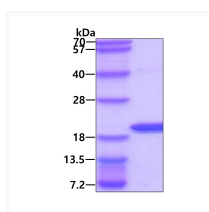
SDS-PAGE gel of recombinant human AG-3 protein 3µg under reducing conditions stained with Coomassie blue
