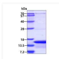
SDS-PAGE gel of recombinant human CDC26 protein 3µg under reducing conditions Coomassie blue stain
