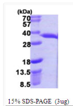
SDS-PAGE gel of recombinant E. coli hchA protein 3 µg under reducing conditions stained with Coomassie blue
