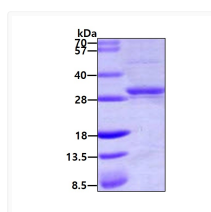
SDS-PAGE gel of recombinant human CMPK1 protein under reducing conditions Coomassie blue stain
