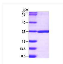
SDS-PAGE gel of recombinant human NUDT16L1 SDOS protein under reducing conditions Coomassie blue stained
