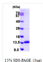
SDS-PAGE gel of recombinant human SNRPE protein 3ug under reducing conditions with Coomassie blue stain
