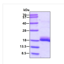
SDS-PAGE gel of recombinant human Calcineurin B protein 3µg Coomassie stain
