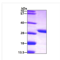
SDS-PAGE of recombinant human AK4 protein under reducing conditions with Coomassie blue stain
