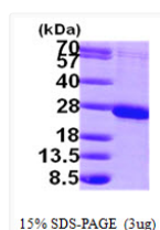
SDS-PAGE gel showing recombinant human RAB1B protein under reducing conditions with Coomassie blue stain
