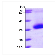
SDS-PAGE gel of recombinant human CDKN3 protein under reducing conditions stained with Coomassie blue
