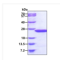
SDS-PAGE gel of recombinant human MDP1 protein 3µg reducing conditions Coomassie blue stain
