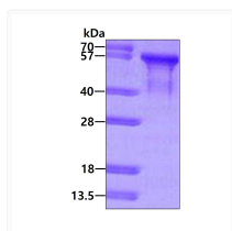
SDS-PAGE of recombinant human Tau 381 1N3R MAPT protein under reducing conditions
