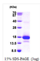
SDS-PAGE gel of recombinant human MCEE protein under reducing conditions stained with Coomassie blue
