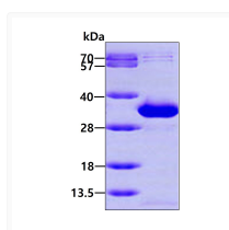
SDS-PAGE gel of recombinant human HDHD4/NANP protein under reducing conditions stained with Coomassie blue
