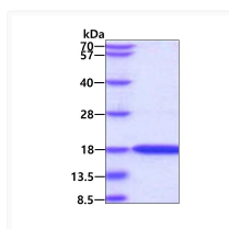
SDS-PAGE gel showing recombinant human LC3A MAP1LC3A protein 3µg under reducing conditions Coomassie blue stain
