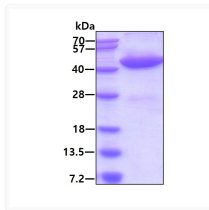
SDS-PAGE of recombinant human GALK1 protein under reducing conditions Coomassie blue stain
