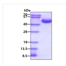
SDS-PAGE of recombinant human ASS1 protein under reducing conditions with Coomassie blue stain
