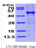
SDS-PAGE gel of recombinant human FKBPL protein under reducing conditions stained with Coomassie blue
