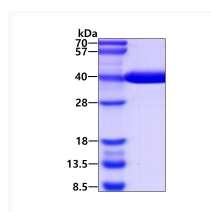
SDS-PAGE gel of recombinant human LDHB protein stained with Coomassie blue under reducing conditions
