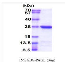
SDS-PAGE gel of recombinant human UBE2T protein under reducing conditions stained with Coomassie blue
