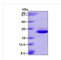
SDS-PAGE gel of recombinant human H-Ras protein 3µg under reducing conditions Coomassie blue stain
