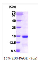
SDS-PAGE gel of recombinant human eIF-1A/EIF1 protein under reducing conditions
