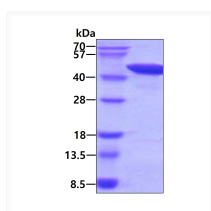
SDS-PAGE gel of recombinant human FEN1 protein 3µg under reducing conditions Coomassie blue stain
