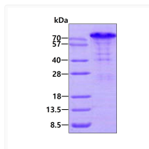
SDS-PAGE gel of recombinant human BAG3 protein under reducing conditions Coomassie blue stain
