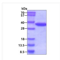
SDS-PAGE of recombinant human Annexin A5 ANXA5 protein under reducing conditions
