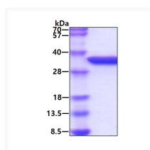
SDS-PAGE gel of recombinant human NQO1 protein stained with Coomassie blue
