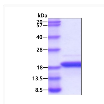
SDS-PAGE gel of recombinant human 4E-BP1/EIF4EBP1 protein under reducing conditions stained with Coomassie blue
