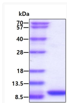
SDS-PAGE gel of recombinant human CCL5 RANTES protein under reducing conditions
