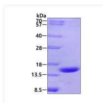
SDS-PAGE of recombinant human Chromogranin A CHGA protein under reducing conditions
