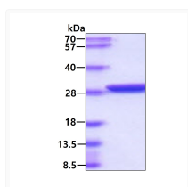
SDS-PAGE gel of recombinant Aequorea victoria GFP protein 3 µg under reducing conditions Coomassie blue stain
