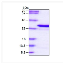
SDS-PAGE gel of recombinant human AK4 C22S protein under reducing conditions stained with Coomassie blue
