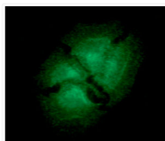
ICC IF of PA2G4 in A549 cells with DAPI and Alexa Fluor 488 staining
