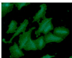
ICC IF of PA2G4 in HeLa cells with DAPI and Alexa Fluor 488 staining
