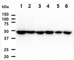
Western blot of human PA2G4 antibody in HeLa, MCF7, A549, 293T, A431 and Jurkat cell lysates
