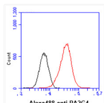
Flow cytometry of PA2G4 in HeLa cells with goat anti-mouse IgG Alexa Fluor 488
