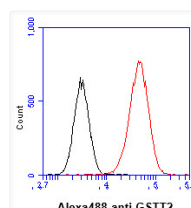
Flow cytometry of GSTT2 in HeLa cells with goat anti-mouse IgG Alexa Fluor 488 conjugate
