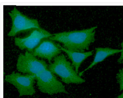
ICC IF of GSTT2 in HeLa cells with DAPI and Alexa Fluor 488 staining
