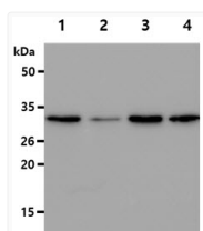
Western blot of human GSTT2 protein expression in multiple cell lines using STJA0041766 antibody
