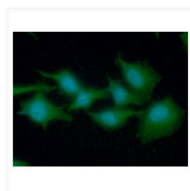
ICC IF of EEF1A1 in A549 cells stained with STJA0041724 antibody Alexa Fluor 488 green and DAPI blue
