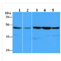
Western blot of Human EEF1A1 antibody across multiple cell lines using anti-mouse HRP detection
