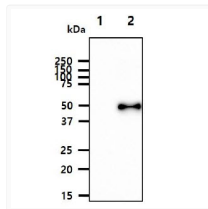
Western blot of recombinant human Aurora kinase B with anti-human Aurora B antibody
