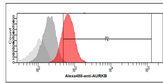
Flow cytometry of Aurora B in LNCaP cells using STJA0041592 antibody with Alexa Fluor 488 detection
