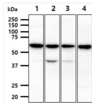
Western blot of human FLIP protein in Jurkat HeLa MCF7 and K562 cell lysates
