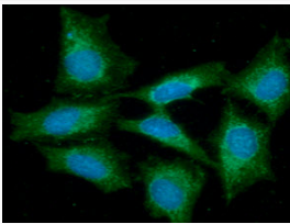
ICC IF of FLIP protein in HeLa cells stained with STJA0041491 antibody and Alexa Fluor 488
