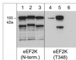
Western blot anti-eEF2K antibody phosphorylation states in recombinant human eEF2K STJA0041211
