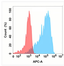
B7H4 antibody flow cytometry Expi293 cells transfected STJA0038118
