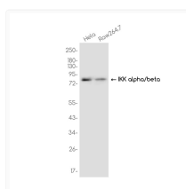
IKK alpha/beta antibody western blot HeLa Raw2647 STJA0037518
