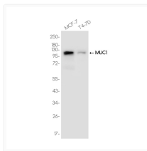
MUC1 antibody western blot MCF-7 T4-7D lysates STJA0037476
