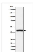
CD1c antibody western blot Jurkat cells STJA0037447
