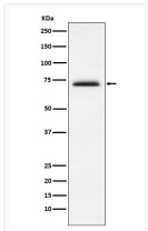
FXR1 antibody western blot MCF-7 cells STJA0037347
