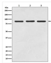
STAT5 antibody western blot Jurkat 3T3 PC-12 STJA0036151
