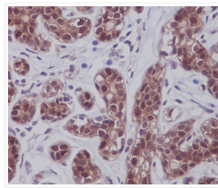
STAT5A/B antibody immunohistochemistry human breast STJA0036151
