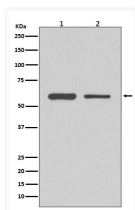
CDK8 antibody western blot HeLa 3T3 lysates STJA0036121
