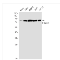
SUZ12 antibody western blot HeLa A549 MCF-7 293T C2C12 STJA0035373
