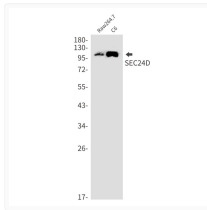
SEC24D antibody western blot Raw2647 C6 STJA0035358
