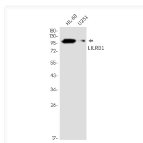
LILRB1 antibody western blot HL-60 U251 STJA0035253
