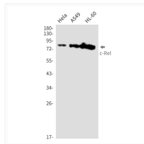
c-Rel antibody western blot HeLa A549 HL-60 STJA0035164
