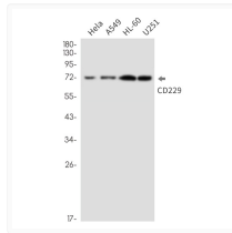
CD229 antibody western blot HeLa A549 HL-60 U251 STJA0035148
